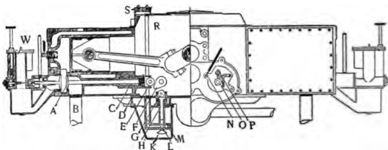
FIG. 398.—Sectional Diagram of the Winton Two-cylinder Horizontal Engine, showing details of valves and oil pump. A, exhaust valve; B, pipe leading exhaust gases to muffler; C, exhaust valve spring; D, set screw; E, roller engaging cam, F, which also engages with roller, G, and operates oil pump piston, H; K, filter for oil forced from pump; L, ball valve on oil pump; M, by-pass for excess of oil from pump; N, primary wire from coil to breaker box; O, spark cam; P, contact adjusting screw; R, vertical pipe for oil forced from pump; S, oil conduit and adjusting screws to regulate flow of parts; W, pin projecting from float in carburetter. This cut also shows the shape and position of the carburetters, of the inlet valve air-line relief pipe, and the sparking plug. The hand wheels and spindles rising from the carburetters serve to regulate the maximum output of gasoline at each suction stroke.
